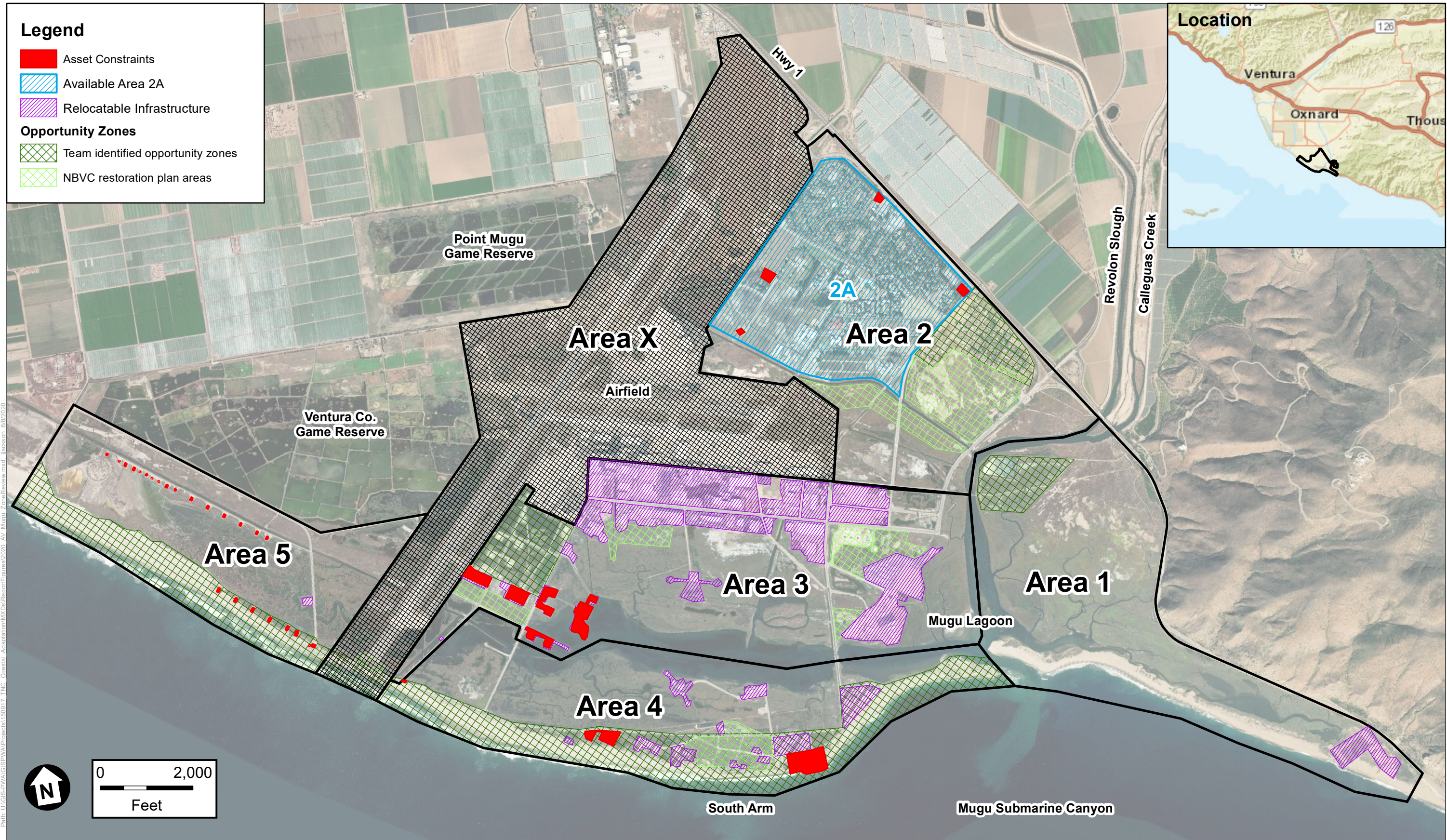
Figure A11 Review of Zones at NBVC Mugu
