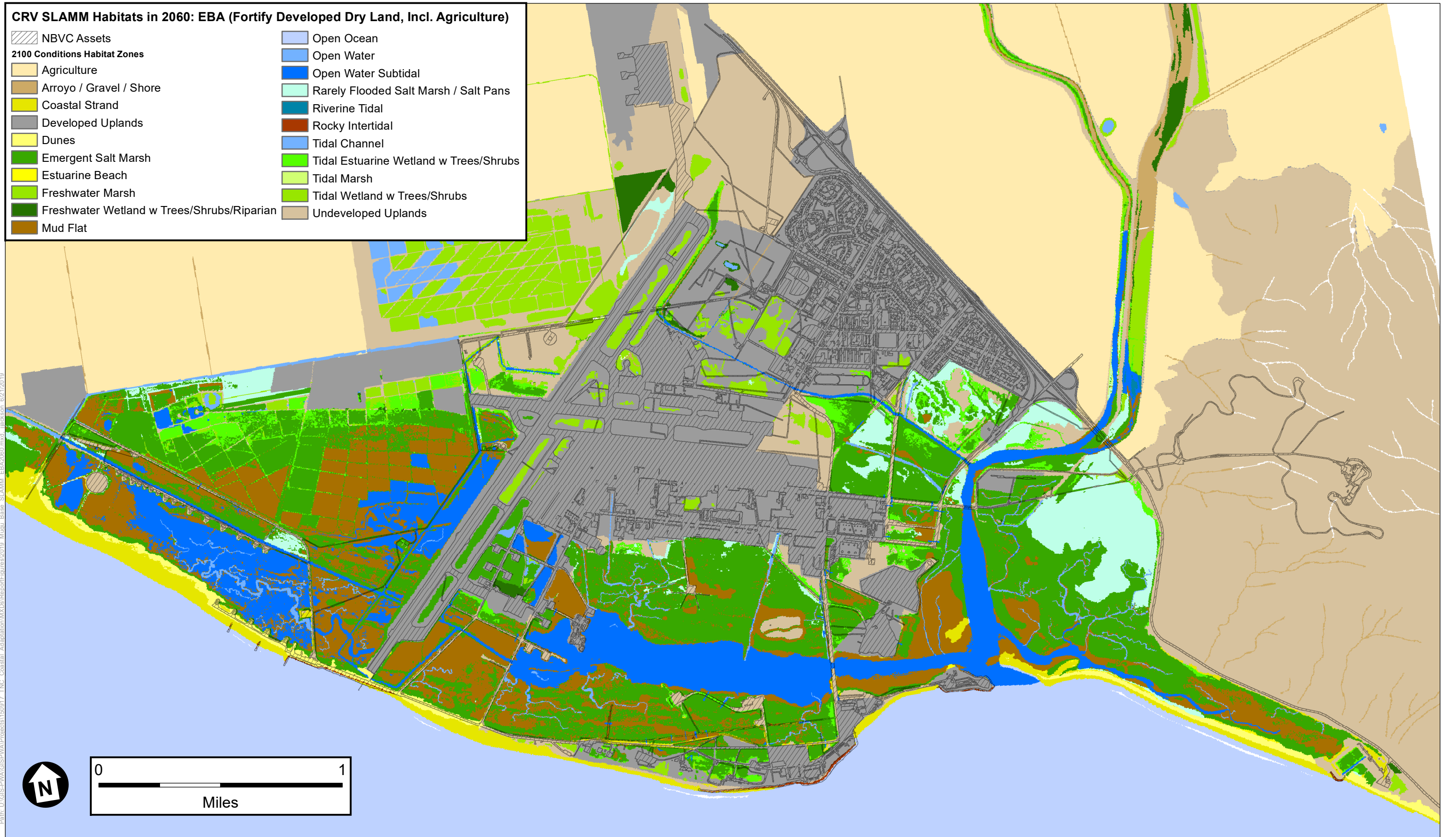
Figure A6 Engineering-Based Adaptation - 2060 Habitats (CRV SLAMM) Fortify Developed Dry Lands (Including Agriculture)
