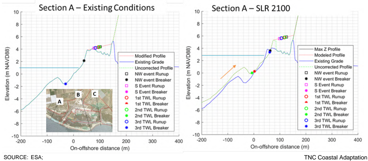
Figure 16 Wave run-up at Section A (Area 5) for existing (left) and future (right) conditions
