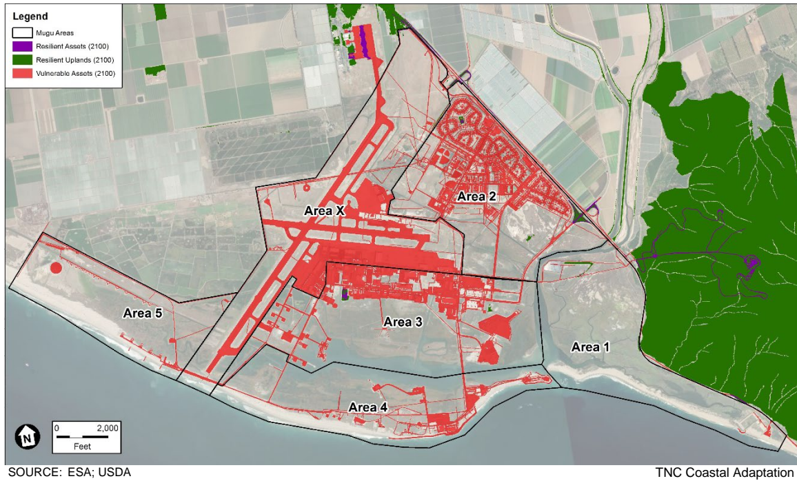
Figure 10 Resilient and Vulnerable Built Assets at NBVC Point Mugu in 2100
