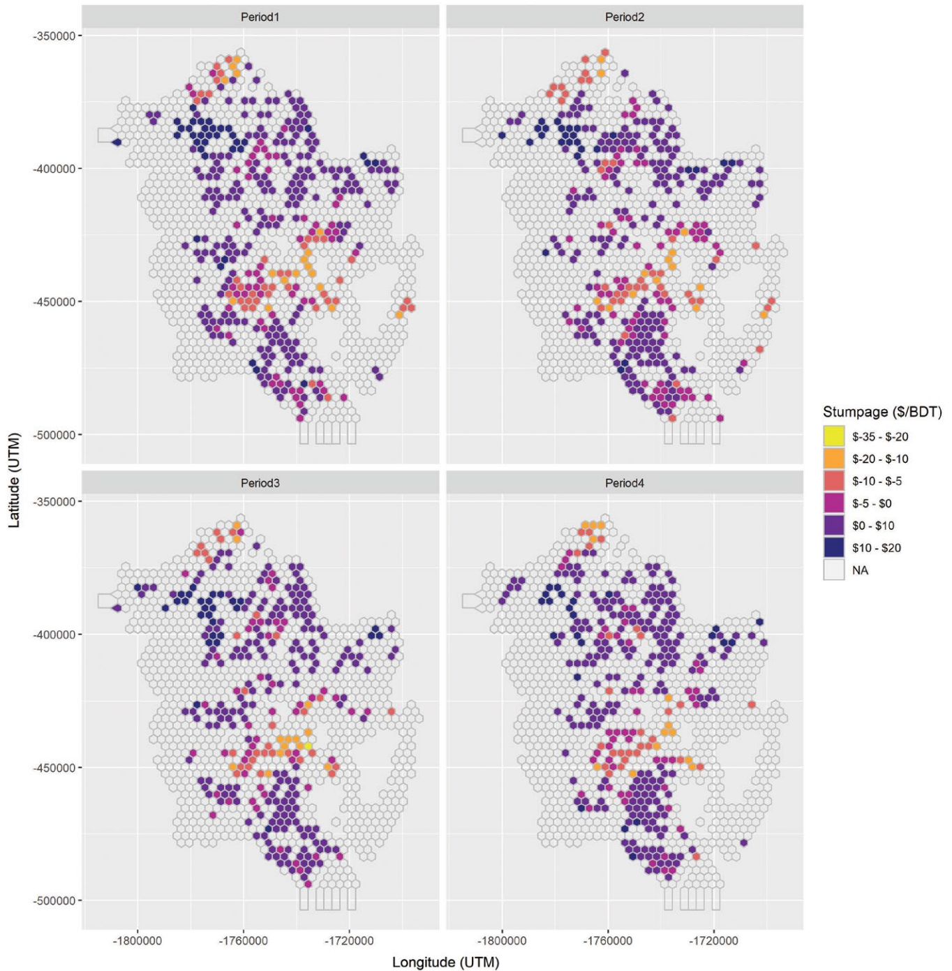
FIGURE 7. Live biomass stumpage for stand-aggregate hexagons in Scenario 1 Case C for each five-year period.
