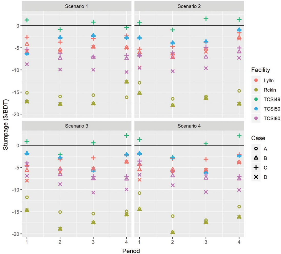
FIGURE 10. Per-unit stumpage for live biomass delivered to each facility, including the existing location at Rocklin (olive green) and the hypothetical locations: reopened Loyalton (salmon), Hwy. 80 near Bowman (pink), Hwy. 50 near Camino (blue), and Hwy. 49 near Camptonville (light green).
