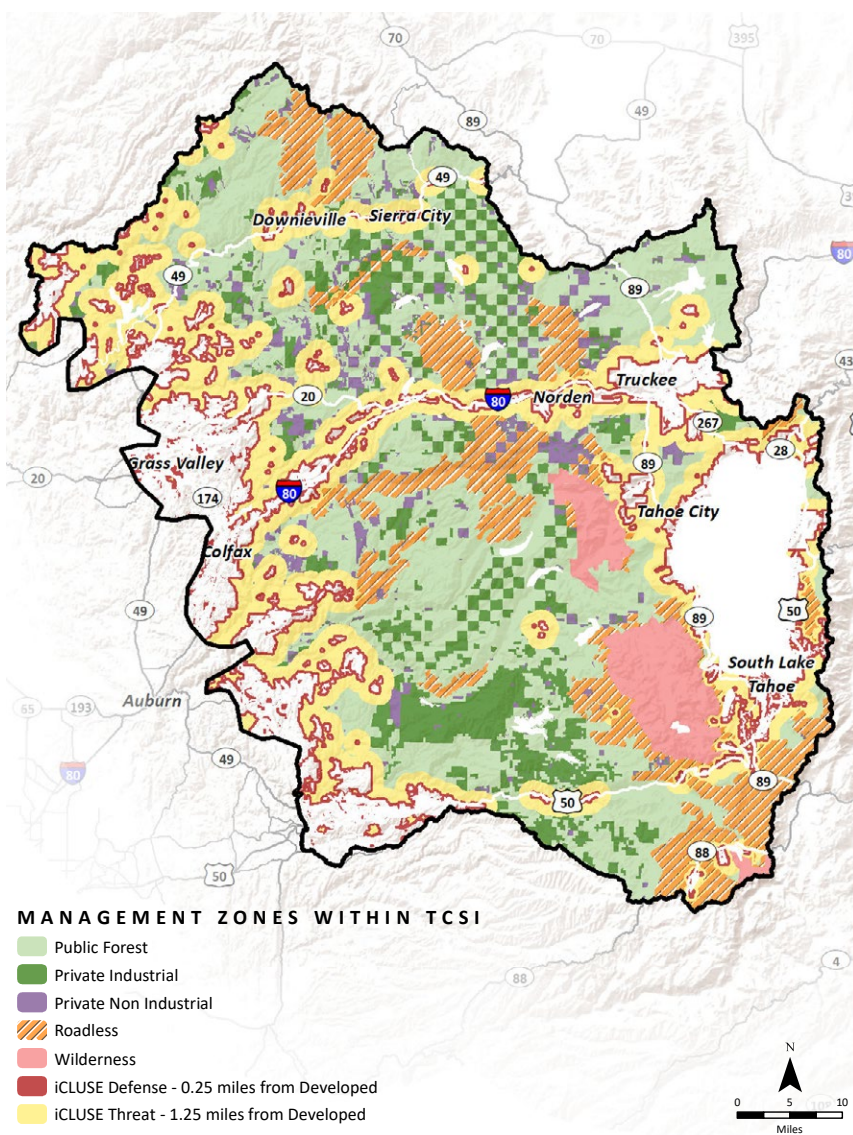
FIGURE 2. Forest management zones for the TCSI region. The iCLUSE Defense and Threat Zones include the Wildland Urban Interface (WUI) surrounding developed areas, including permanent infrastructure (e.g. interstates, highways).
